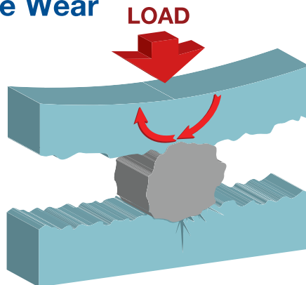
Particle caught, surfaces dented and cracking initiated
