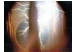
Electrical discharge occurring inside oil tank
