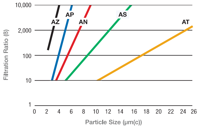
Multi-Pass Filter Ratings (ISO 16889)
