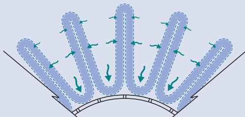
Traditional Fan-Pleat Filter
